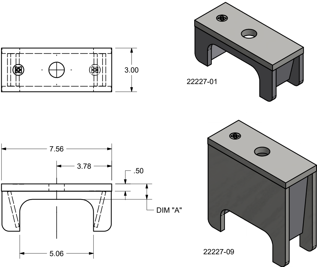
*HEAVY DUTY SPRING SEAT WITH .50 TOP PLATE
