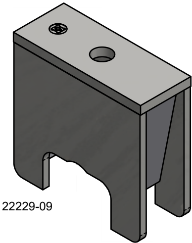
*HEAVY DUTY SPRING SEAT WITH .50 TOP PLATE
