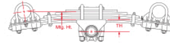
Underslung Axles - Overslung Trunnion
