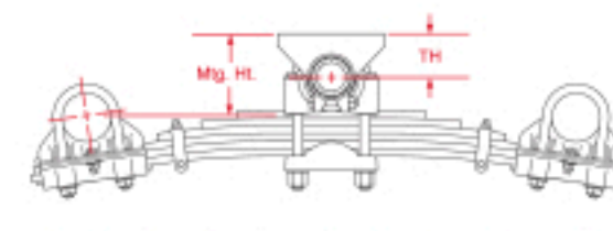
Underslung Axles - Underslung Trunnion
