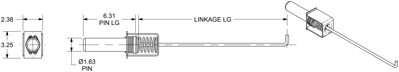
OBSOLETE EZ PULL CARTRIDGE
