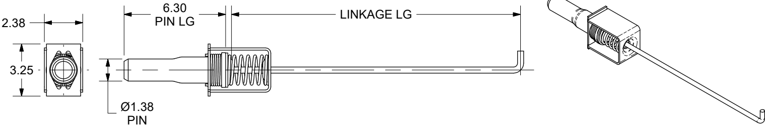
OBSOLETE EZ PULL CARTRIDGE
