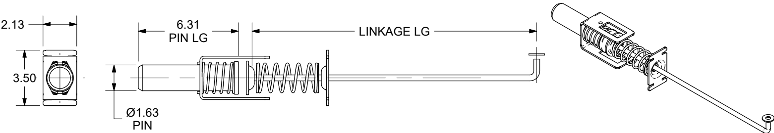
EZ PULL 2 STYLE SERVICE KIT
