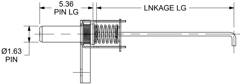
EZ PULL 2 STYLE SERVICE KIT
