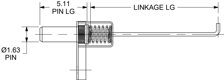
OBSOLETE EZ PULL CARTRIDGE
